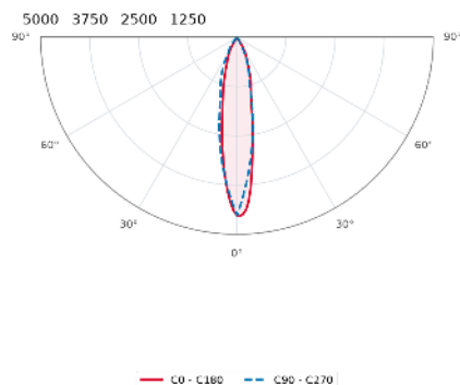
ADL-S IP54 Trimless Downlight • Photometrics
